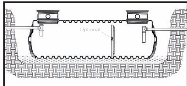
FIG.3 Plumbing Install
